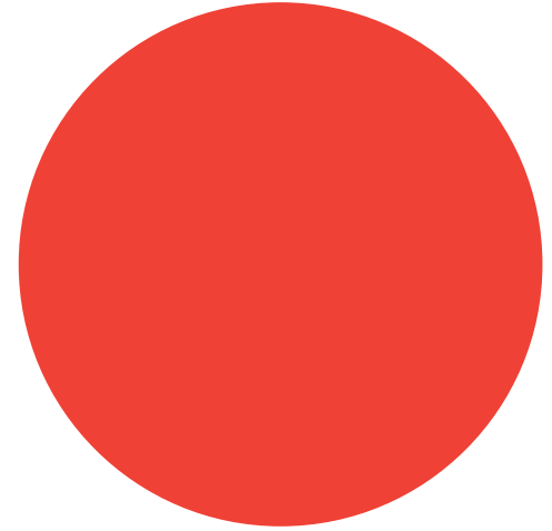
Cinnabar
