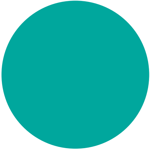
Persian Green
