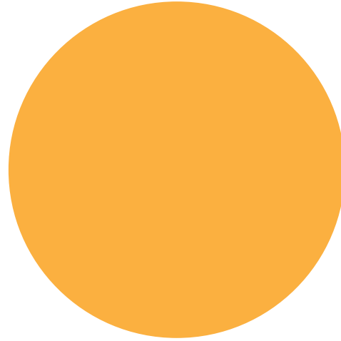
Yellow Orange
